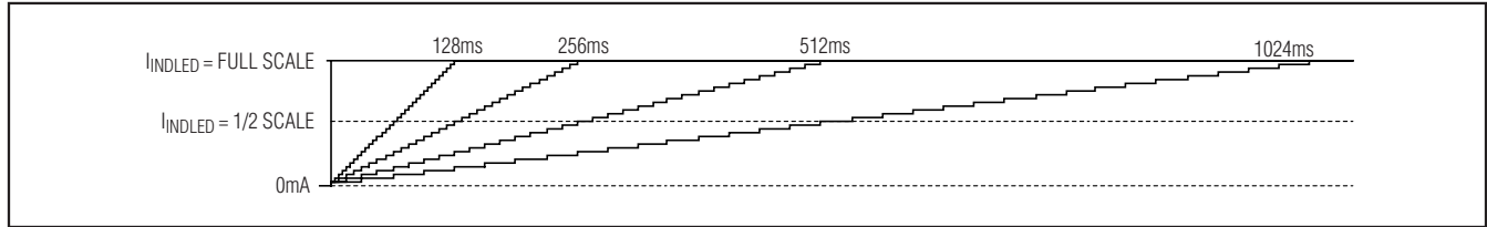
Figure 5. Ramp-Up Behavior
