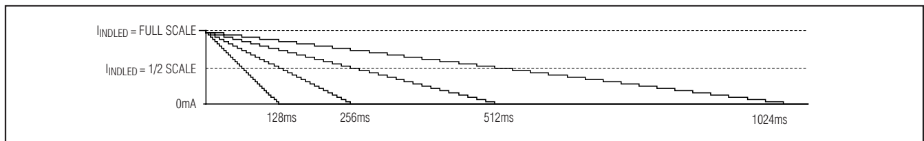
Figure 6. Ramp-Down Behavior
