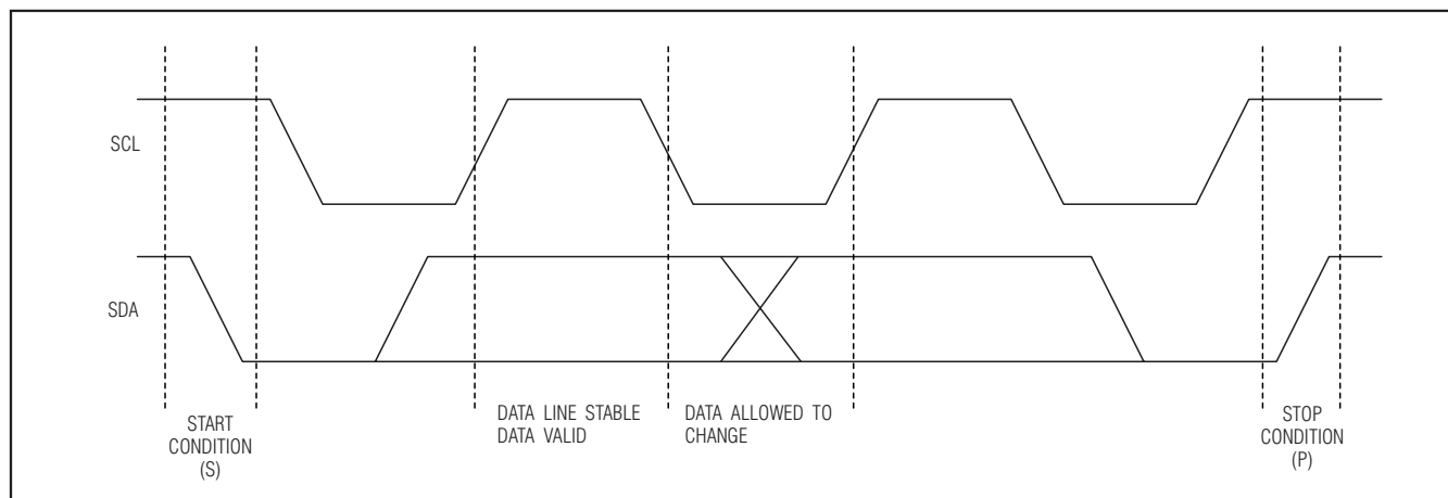
Figure 16. Bit Transfer
